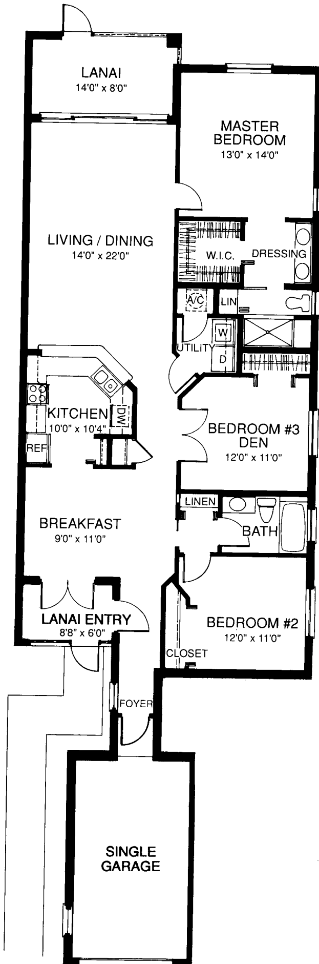
Plan C 3 Bedroom/2 Bath (First Floor)
